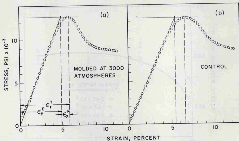
Fig. 4. Typical compressive stress-strain curves for polystyrene glasses: (a) molded at 3000 atmospheres; (b) compression-molded control. Separation of yield strain into \epsilon_y^E and \epsilon_y^P is explained in text.
